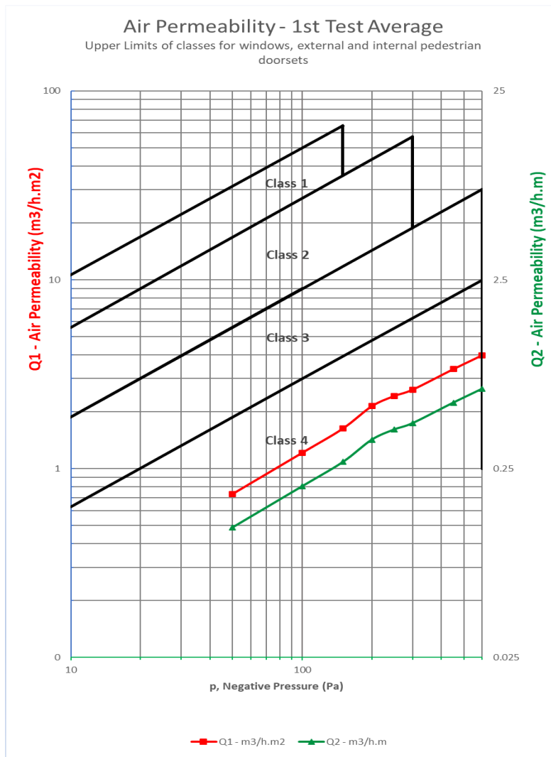
Figure 1: Upper limits of classes for windows and pedestrian doorsets. STIRA Manual Cosy+ Loft Ladder System (Attic Hatch) tested to max test pressure of 600Pa (as required by Class 4).
